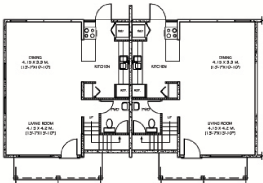
② TWO BEDROOM TOWNHOUSE FLOOR PLAN SCALE: 1:50
