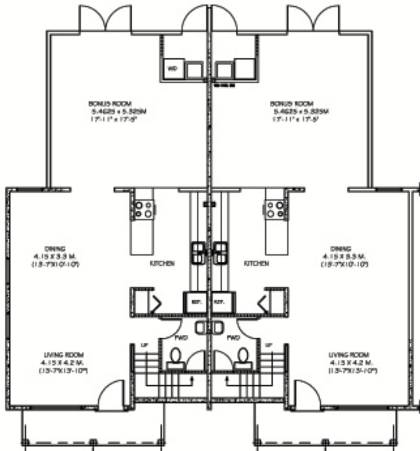
2 THREE BEDROOM LOWER FLOOR PLAN SCALE: 1:50
