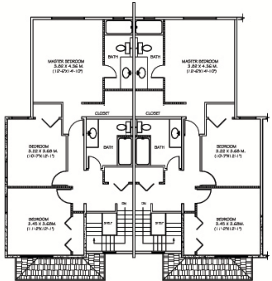
3 THREE BEDROOM UPPER FLOOR PLAN SCALE: 1:50
